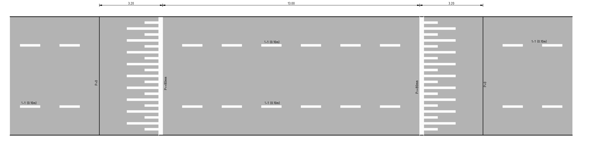
Principedetail plateau 60km/h (h=80mm) Bubeko Schaal 1:50
